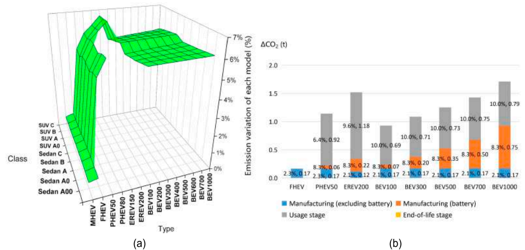
Figure 1. The influence of power grid emission on each type of vehicle. (a) Sensitivity analysis of power grid emission. (b) The emission distribution of different sources (A-class SUV). The numbers are emission reduction amount according to \Delta CO_2 (t) and the percentage is the rate of emission in the corresponding stage (reduced carbon emissions/original carbon emissions).
